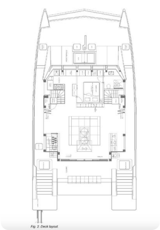
Fig. 2. Deck layout.
