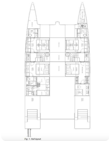
Fig. 1. Hull layout.
