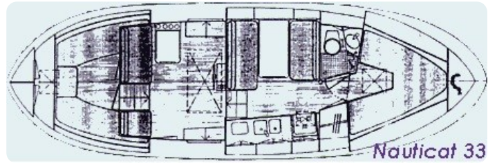
Nauticat 33 _ Layout
