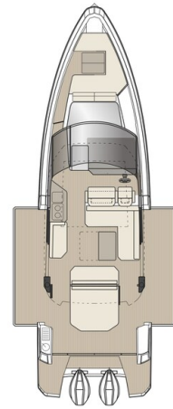
SAXDOR 400 GTC Terrace Layout
