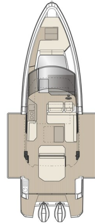
SAXDOR 400 GTC Terrace Layout
