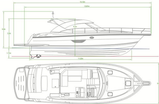
R4400SY Principal Dimensions ISO 8666:2002
