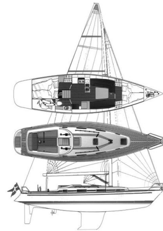
nordborg_40_drawing
