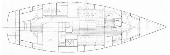
Layout HR 382
