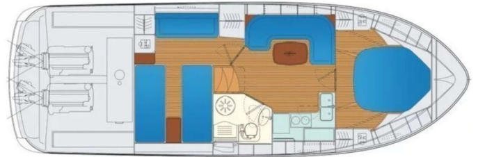
Bavaria 37 Sport_Layout
